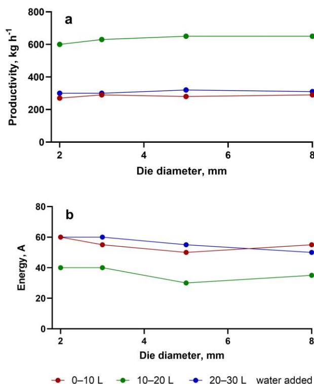
Figure 1. a) Effect of die diameter and water addition on (a) productivity (kg h -1 ) and (b) energy consumption (A) during extrusion of enriched feed additive. Lines show water addition levels: 0-10 L, 10-20 L, and 20-30 L per batch
